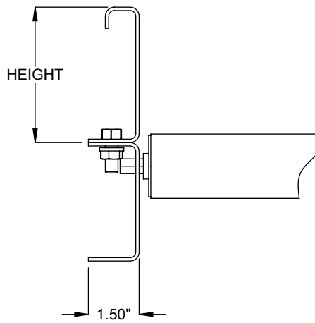
GUARDRAIL
